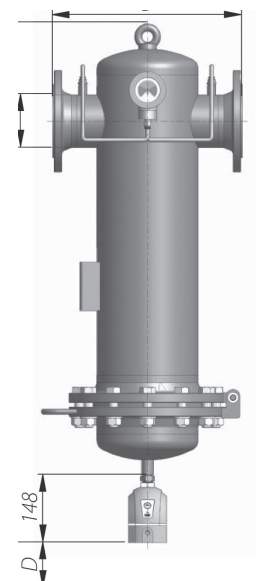
Timer Drain
