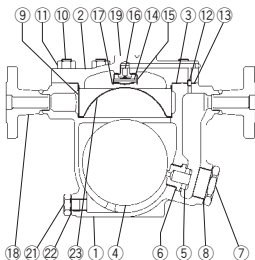
JH7.5R-X
