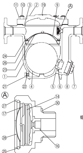
JH7.5R-X
